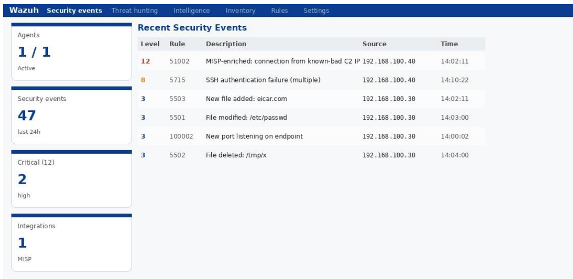
Figure 11 - Wazuh Dashboard home at https://192.168.100.20:8433
